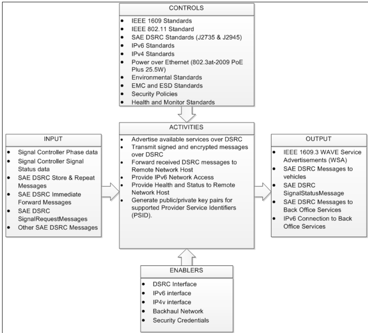
Figure 6: Context diagram of an RSU
