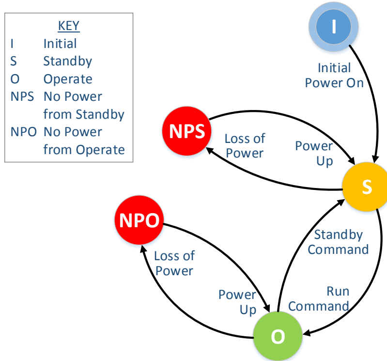
Figure 2: Roadside Unit State Diagram
