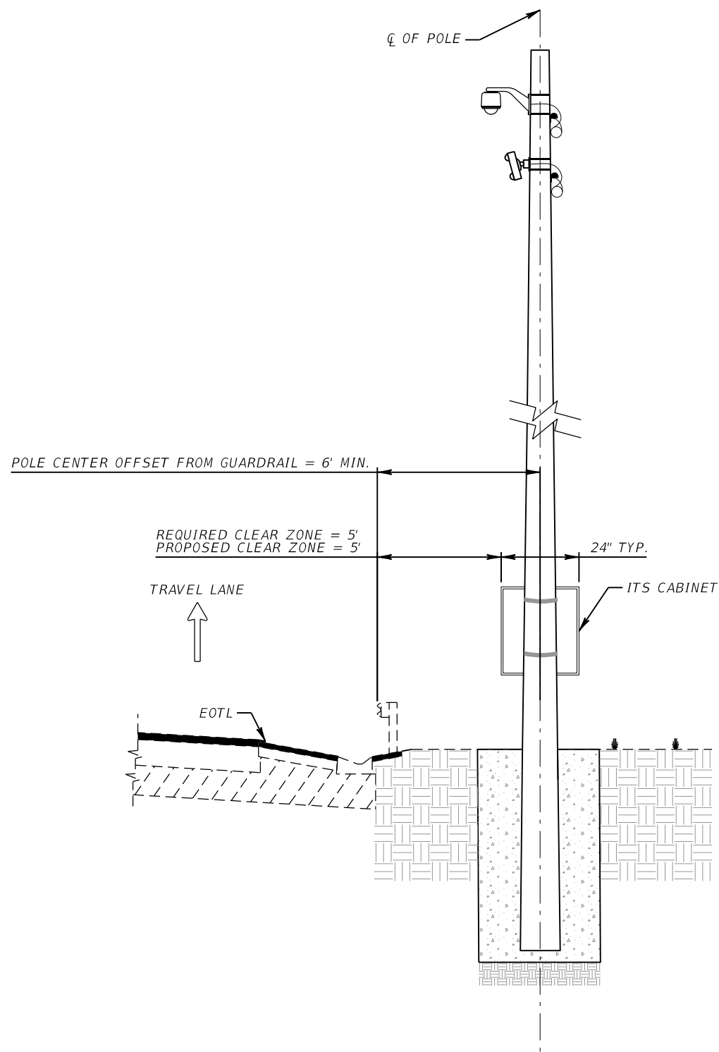
TYPICAL GUARDRAIL CLEAR ZONE DETAIL
