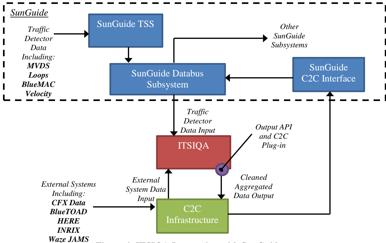
Figure 4: ITSIQA Integration with SunGuide
