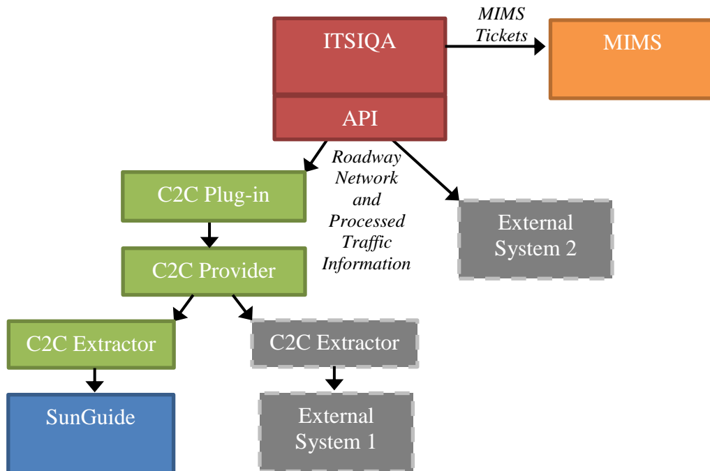
Figure 8: Output ITSIQA Data to Various Systems
